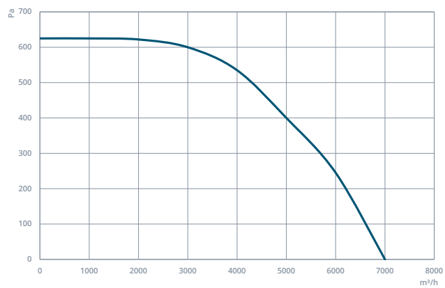
MEF 500
