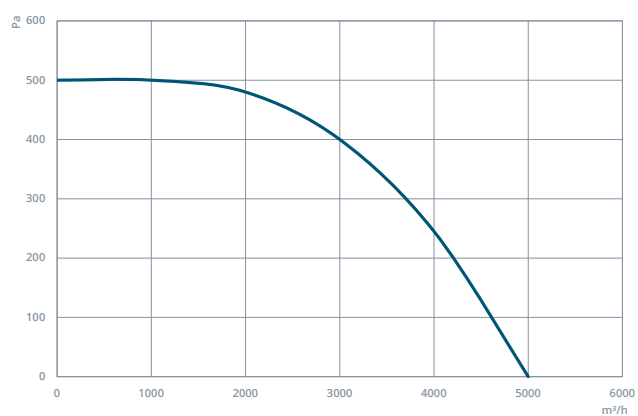
MEF 450
