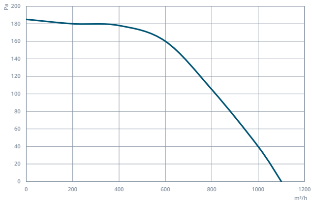
SAL 280
