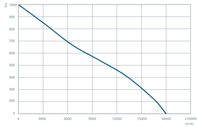
AXI 500-6-45
