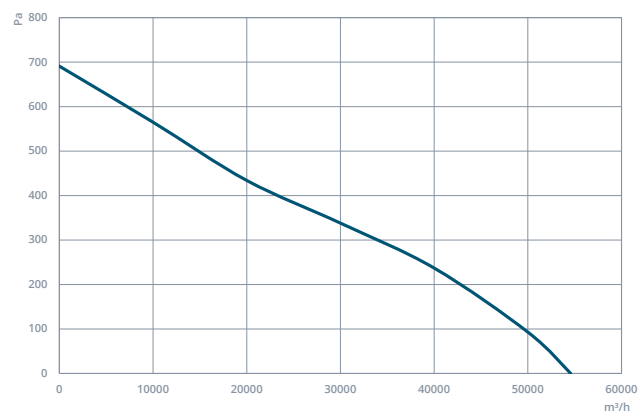
PAXI 1000-5-40
