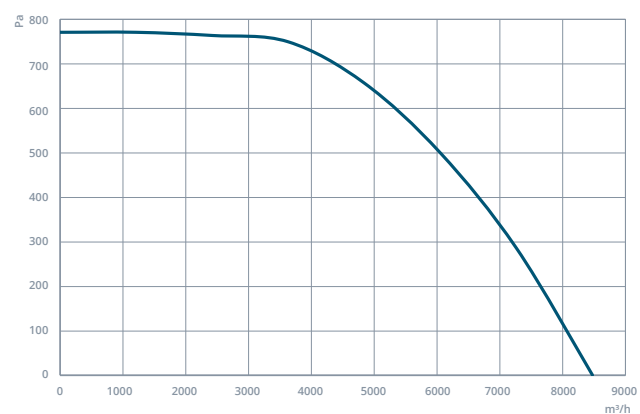
CRADIK 500
