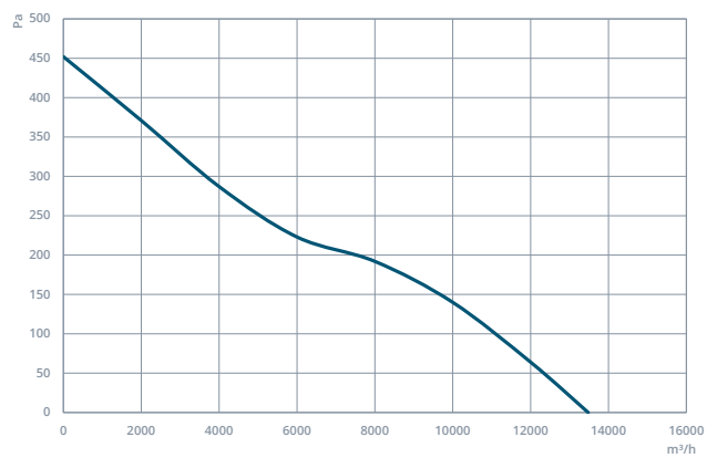
HAXI 630-5-30
