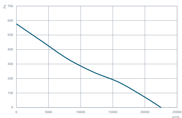
CAXI 800-5-30
