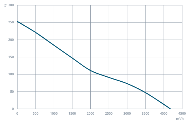
HAXI 450-5-25
