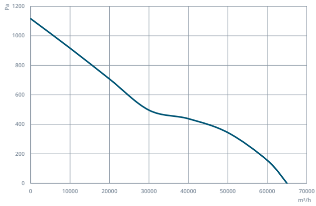
BAXI 1000-8-45
