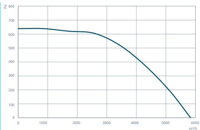
CRADIK 450
