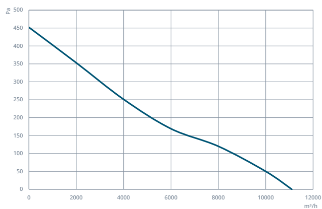
CAXI 630-5-30
