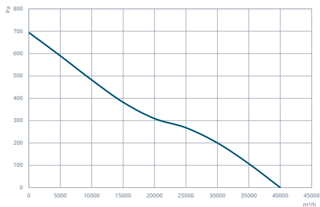
CAXI 900-5-40
