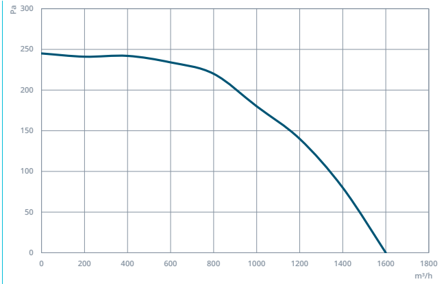
SAL 315
