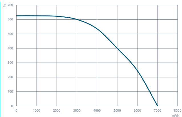
HMEF 500
