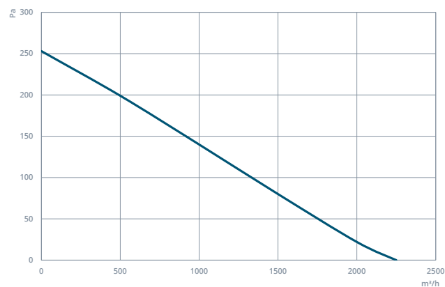
CAXI 450-5-25
