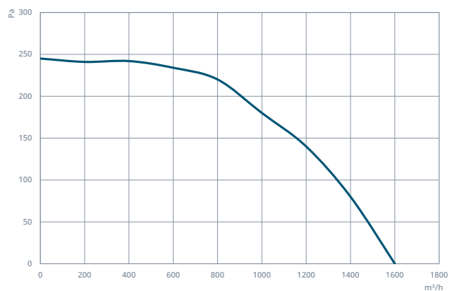
MEF 315
