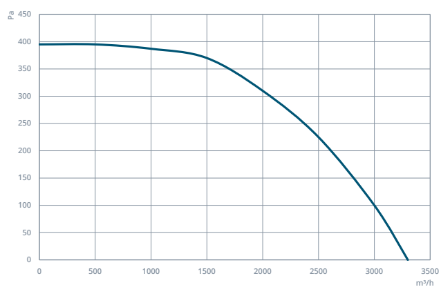
MEF 400
