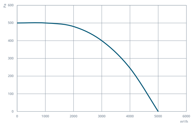
HMEF 450
