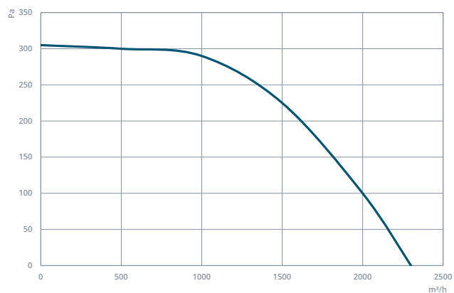
MEF 355
