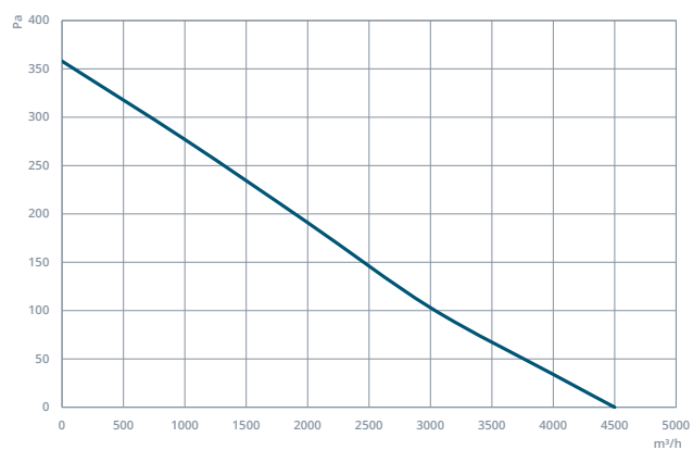
CAXIDIK 560-5-25
