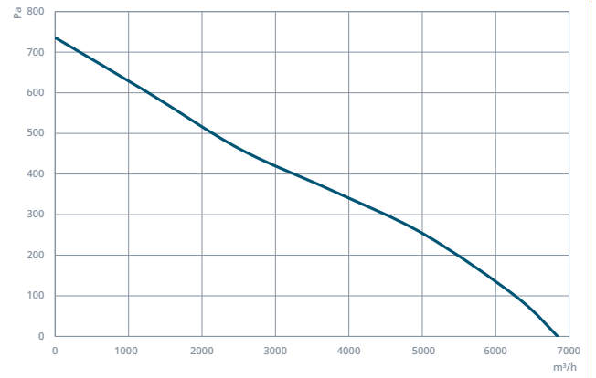
AXI 355-6-45
