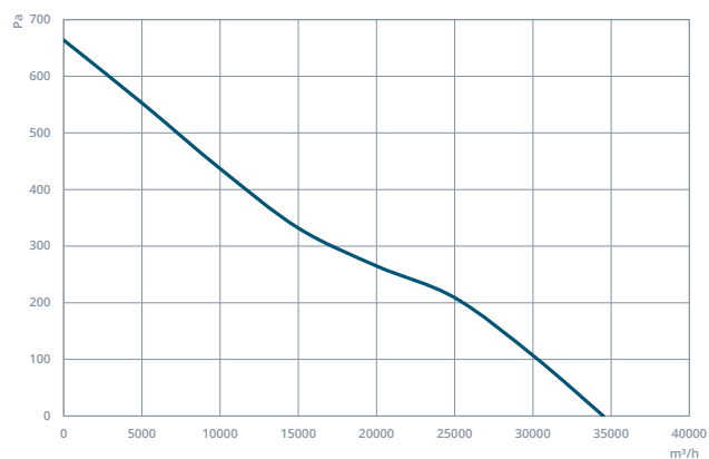
CAXI 900-5-35
