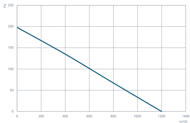
CAXI 400-5-25
