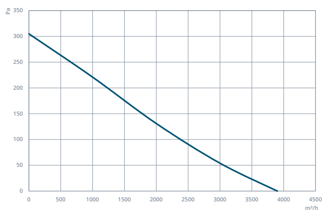
CAXI 500-5-25
