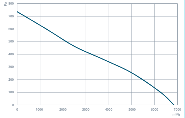
TAXI 355-6-45
